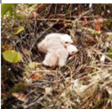
15 Accipiter striatus ACCIPITRIDAE Sharp-shinned Hawk Gavilán pajarero
